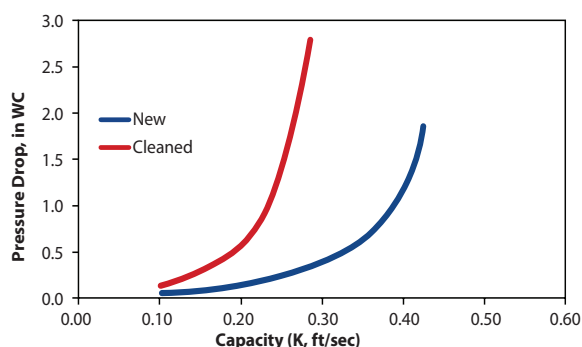
Figure 3. Hydraulic capacity test results show the performance of new versus cleaned mesh. The cleaned mesh was removed from service, cleaned, and reinstalled into pilot plant column for testing.
