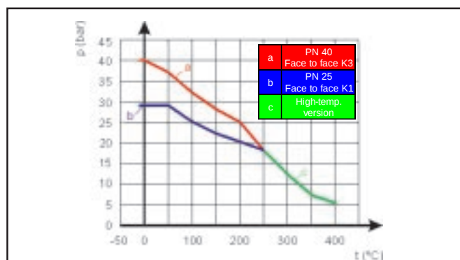
Fig. 6 - Pressure-Temperature diagram
