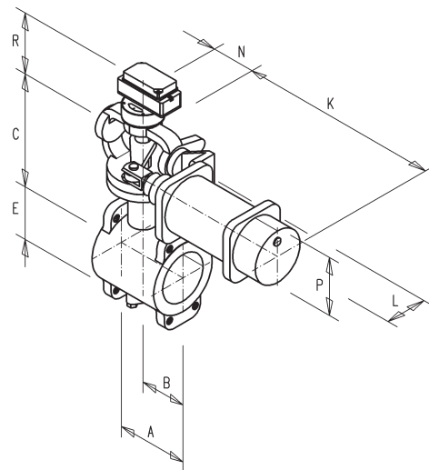
Fig. 8 · Dimensional drawings for VETEC rotary plug valves: Type 72.3 R (flanged design) and Type 72.4 R (wafer-style design)
