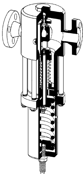
Type 511 B (~ 515 B) bellows control
