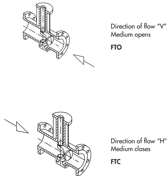
Fig. 4 and 5 · Directions of flow V and H
