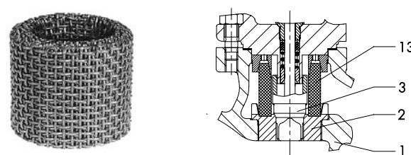
Fig. 2 · St III Flow Divider, installed in Type 3241 Valve
