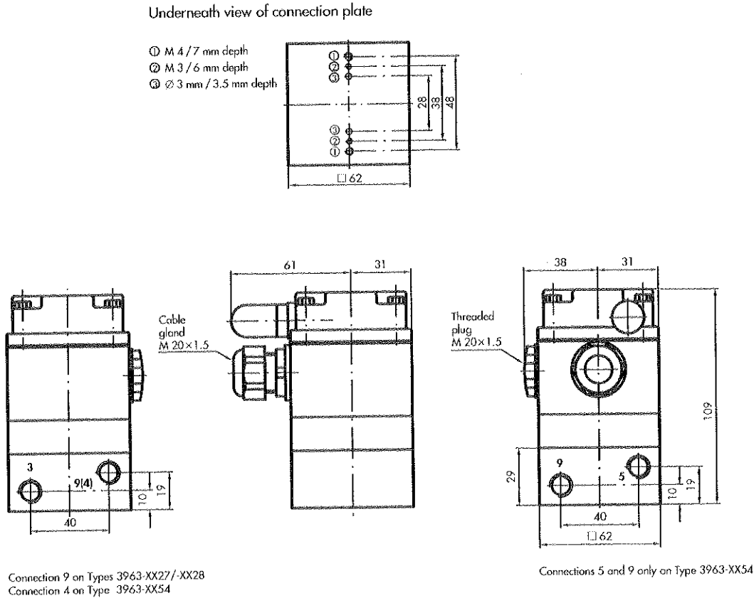
Fig. 20 - Dimensions in mm
