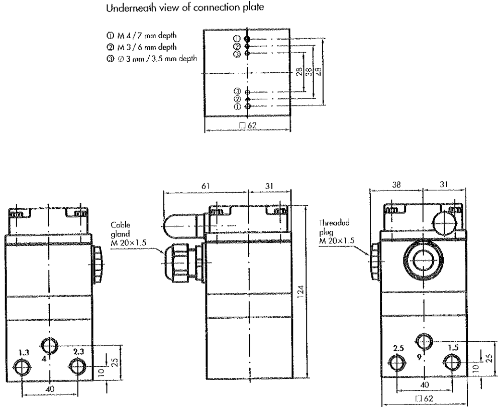
Fig. 19 - Dimensions in mm
