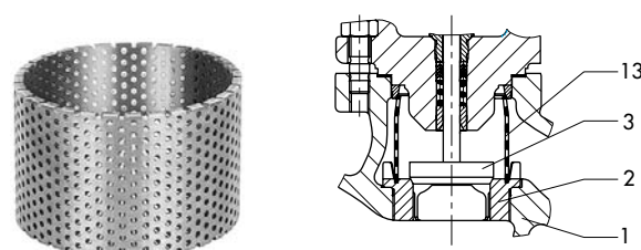
Fig. 1 · St I Flow Divider, installed in Type 3241 Valve
