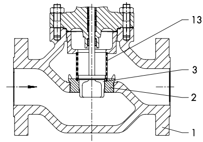
Fig. 4 · Type 3251 Valve with St I Flow Divider
