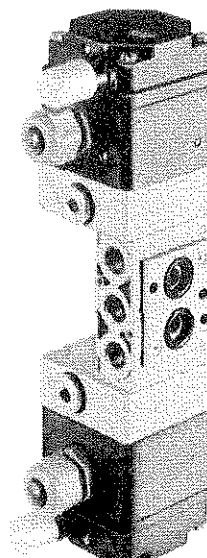
Type 3963-XX76 3/2-way Pilot Valves combined with Type 3756-3327 5/2-way Booster Valve G \frac{1}{4} /NAMUR
