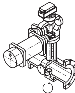
Mounting D-Ps
