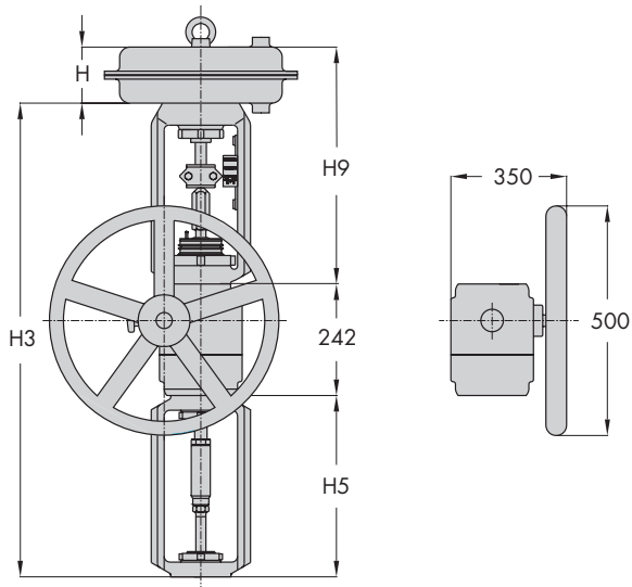
Fig. 19 · Version for 1400 and 2800 cm 2 and a max. of 60 mm of travel with side-mounted handwheel
