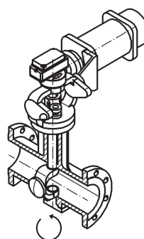
Mounting B-Ps
