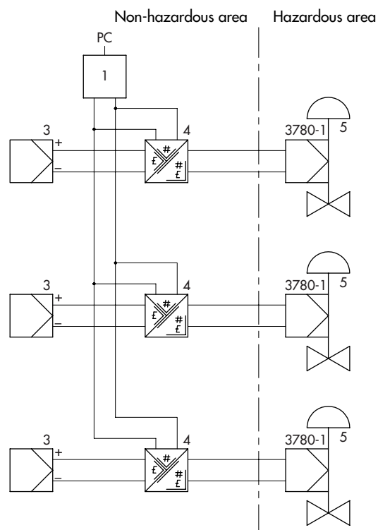
Fig. 9 · Communication over multiplexers illustrated here using a FSK bus
