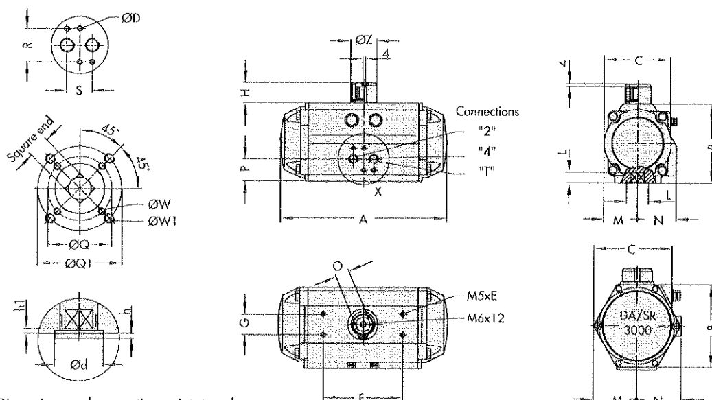
Fig. 4 · Dimensions and connection points to valves
