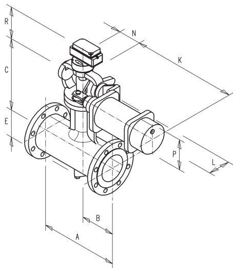
Fig. 8 · Dimensional drawings for VETEC rotary plug valves: Type 72.3 R (flanged design) and Type 72.4 R (wafer-style design)
