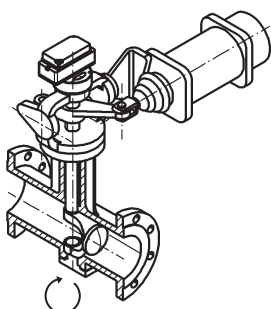
Mounting D-Po
