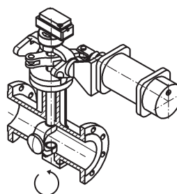
Mounting C-Ps
