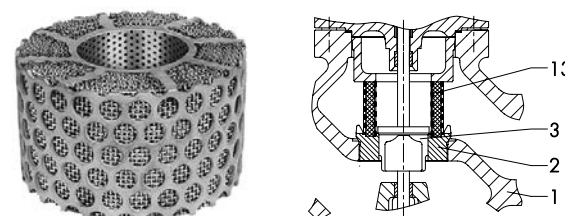
Fig. 3 · St III Flow Divider, installed in Type 3254 Valve
