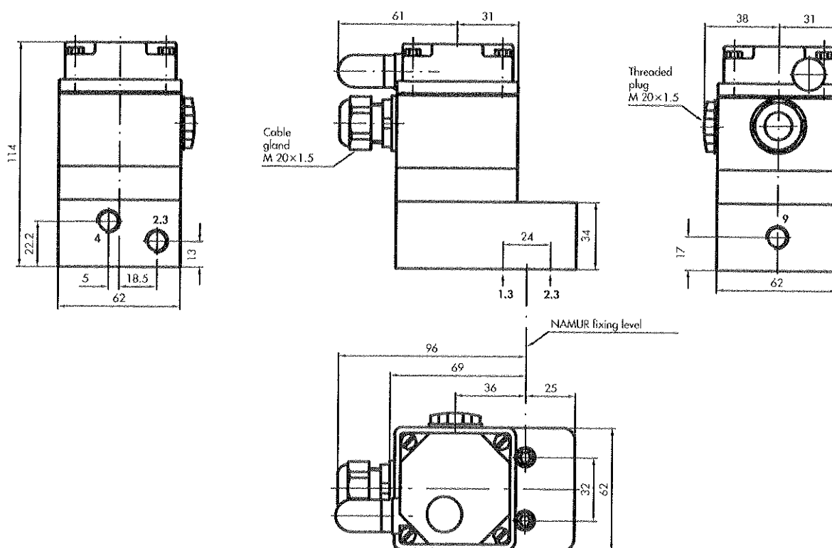
Type 3963-XX52 Solenoid Valve
