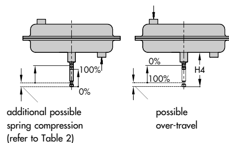
Fig. 12 · Spring compression and travel
