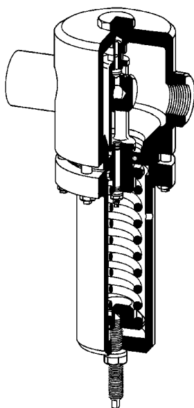
Type 511 B (~ 515 B) bellows control
