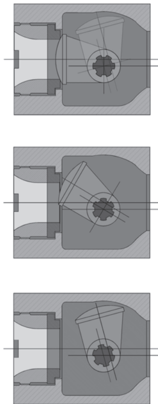
Fig. 3 · Plug movement with double-eccentric bearing
