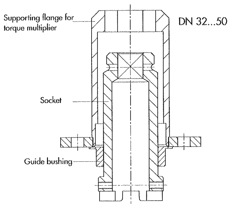
Fig. 7 · Seat wrench 9110-1837
