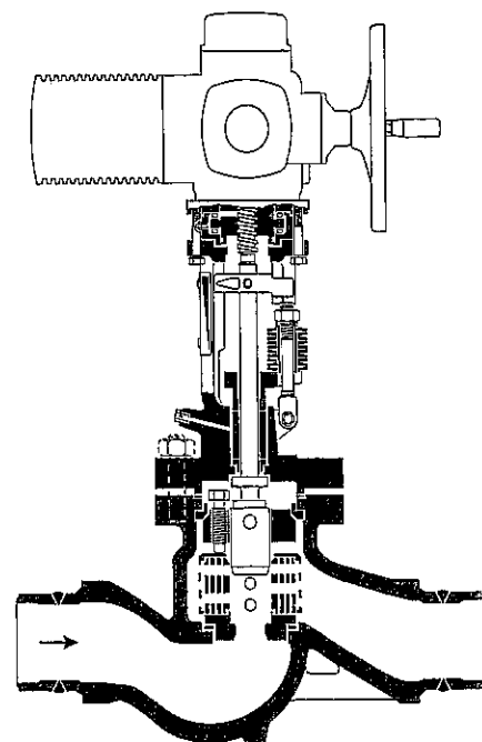
ZK 29/14, DN 80 mm (3") with butt-weld ends
