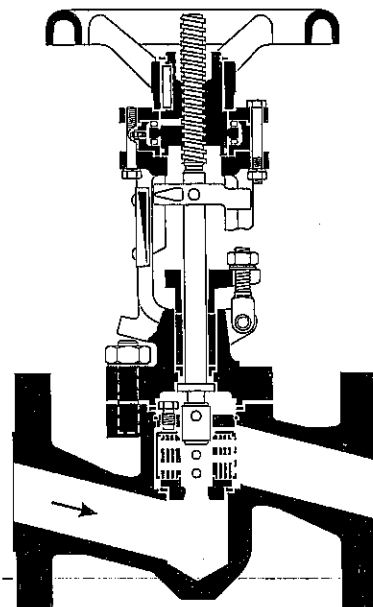
ZK 29/14, DN 25 mm (1") with flanged ends
