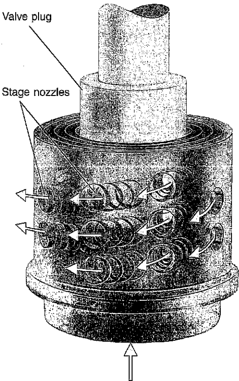
Radial stage nozzle as control unit
