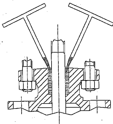
DRAWING N°2
