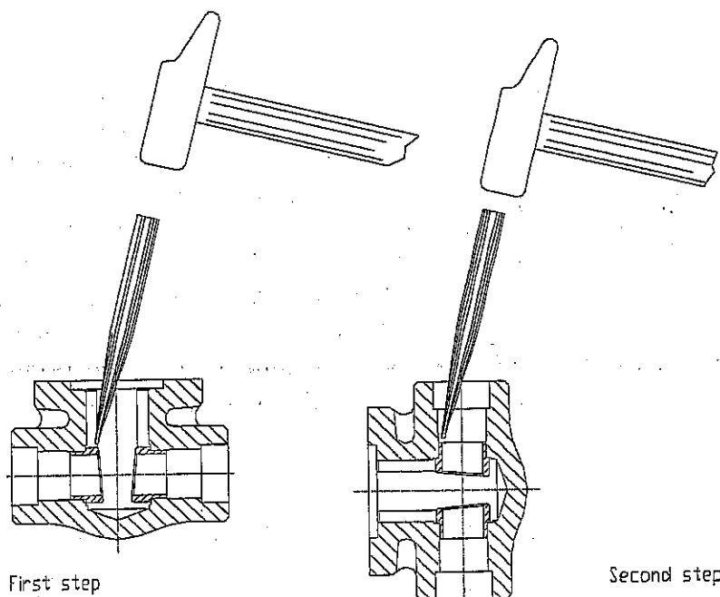
DRAWING N°4
