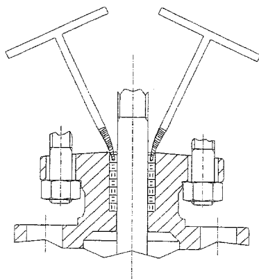
DRAWING N°2
