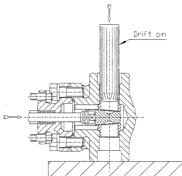
DRAWING N°5
