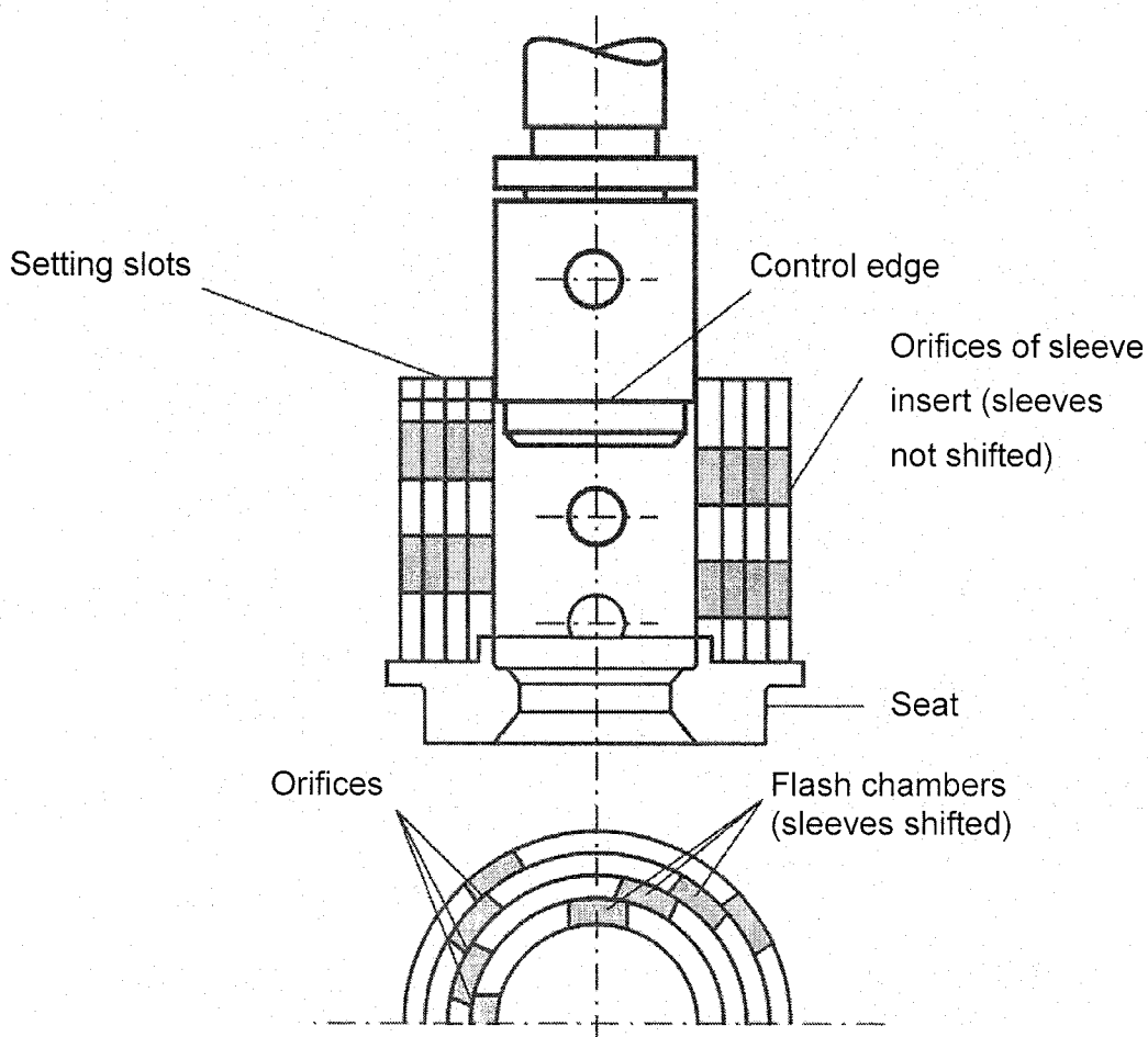
Control valve ZK 29: cross section of the radial stage nozzle
