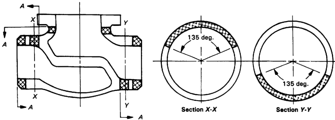
FIG. 11 GLOBE BODY (FLANGED BONNET)
